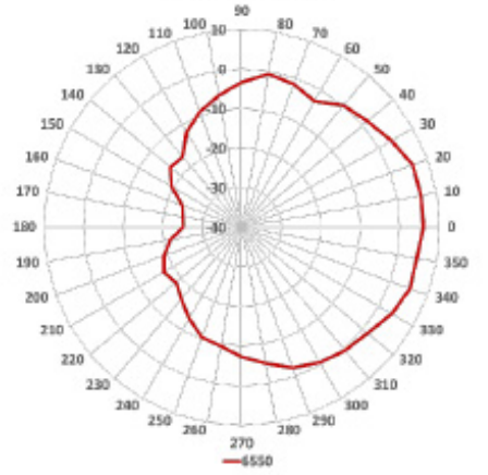
6.0GHz Elevation
