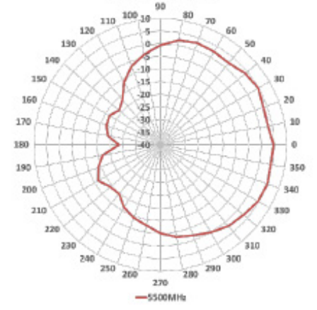
5.0GHz Elevation
