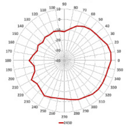
2.4GHz Elevation
