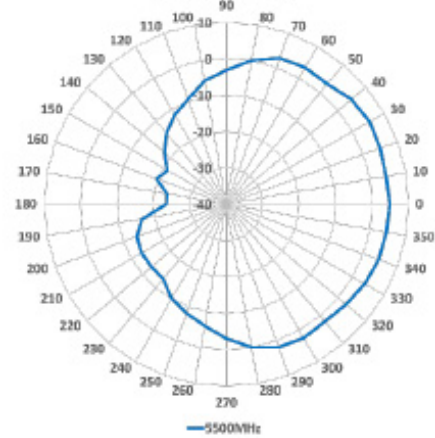
5.0GHz Azimuth
